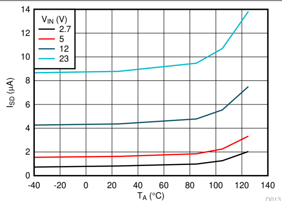
图 7-5. IN Shutdown Current vs Temperature
