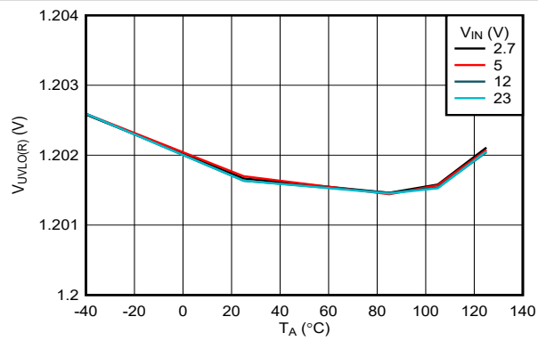
图 7-7. EN/UVLO Rising Threshold vs Temperature
