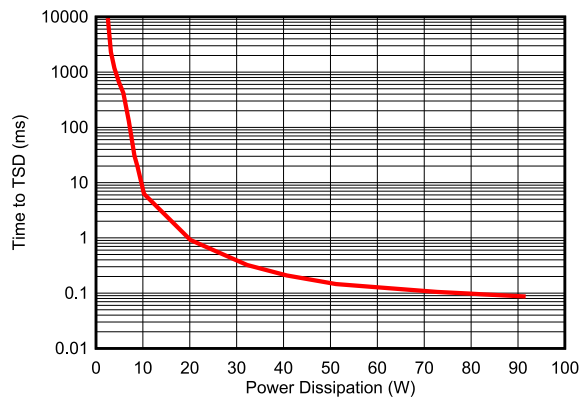
图 7-24. Time to Thermal Shut-Down During Inrush State
