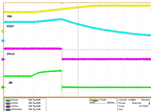
C_{OUT} = 220 \mu F , R_{OUT} = 20 \Omega , V_{IN} Overvoltage threshold set to 13.2 V, V_{IN} ramped up from 12 V to 16 V
