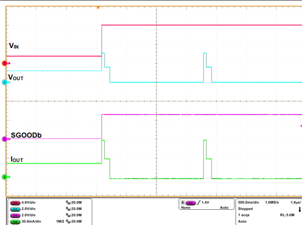
图 7-22. Auto Retry with MODE = 180 kΩ
