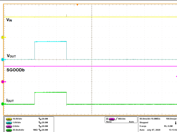
图 7-20. Current Limit with MODE = GND
