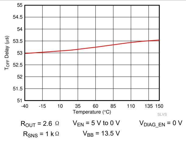
图 7-8. Turn-off Delay Time ( t_{DF} ) vs Temperature
