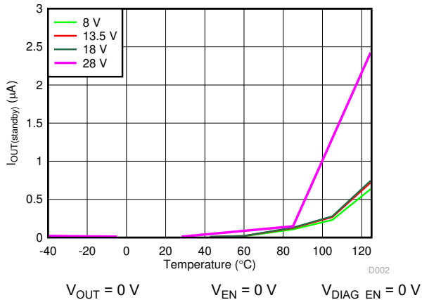
图 7-3. Output Leakage Current ( I_{OUT(standby)} ) vs Temperature
