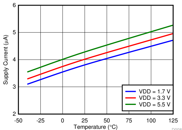
Output ( RESET Pin ) = Low 图 7-10. Supply Current vs Temperature
