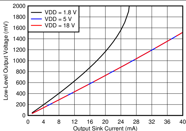
图 5-12. Output Voltage Low ( V_{OL} ) vs Output Sink Current (85°C)
