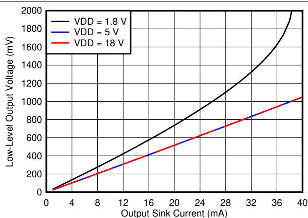
图 5-9. Output Voltage Low ( V_{OL} ) vs Output Sink Current (-40°C)
