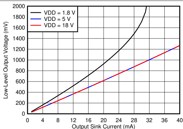
图 5-11. Output Voltage Low ( V_{OL} ) vs Output Sink Current (25°C)
