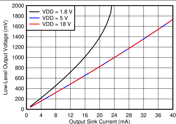
图 5-13. Output Voltage Low ( V_{OL} ) vs Output Sink Current (125°C)
