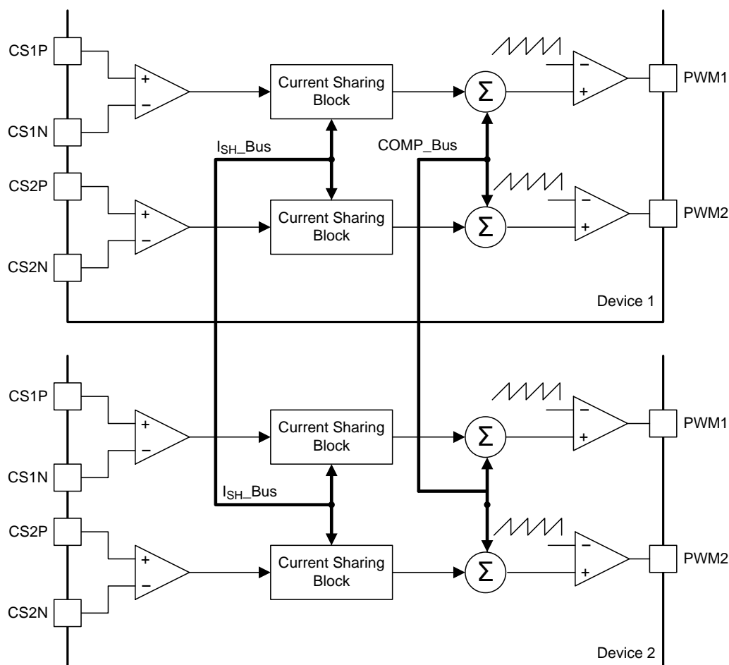
Figure 17. Current Sharing
