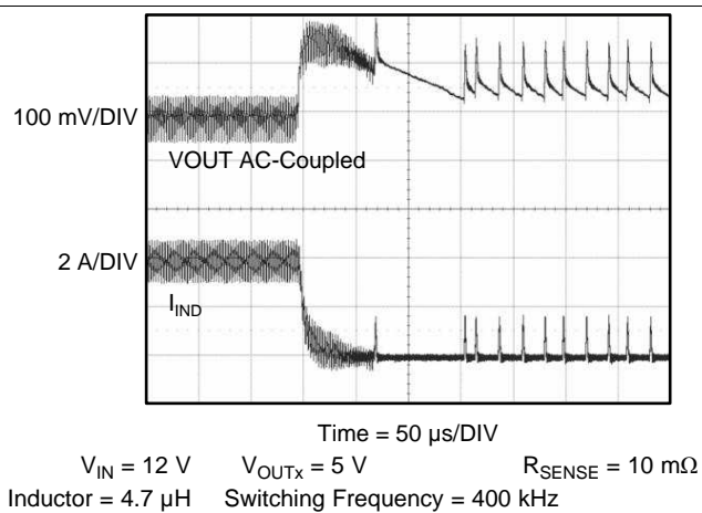
图 5. Buck1 and Buck2 Load Step: Low-Power-Mode Entry (0.09 mA to 4 A at 2.5 A/ \mu\text{s} )
