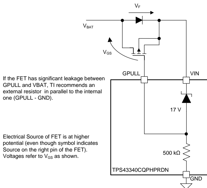
图 15. Internal Circuit of GPULL Output
