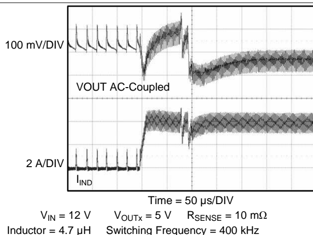
图 6. Buck1 AND Buck2 Load Step: Low-Power-Mode Exit (0.09 mA to 4 A AT 2.5 A/ \mu\text{s} )
