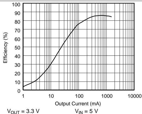
图 1. Buck2 Efficiency versus Output Current Continuous Mode
