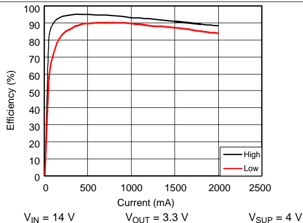
图 2. Buck3 Efficiency vs Output Current, 400 kHz 25°C
