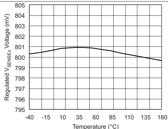
图 4. Regulated V_{SENSEx} Voltage vs Temperature (Buck1 and Buck2)
