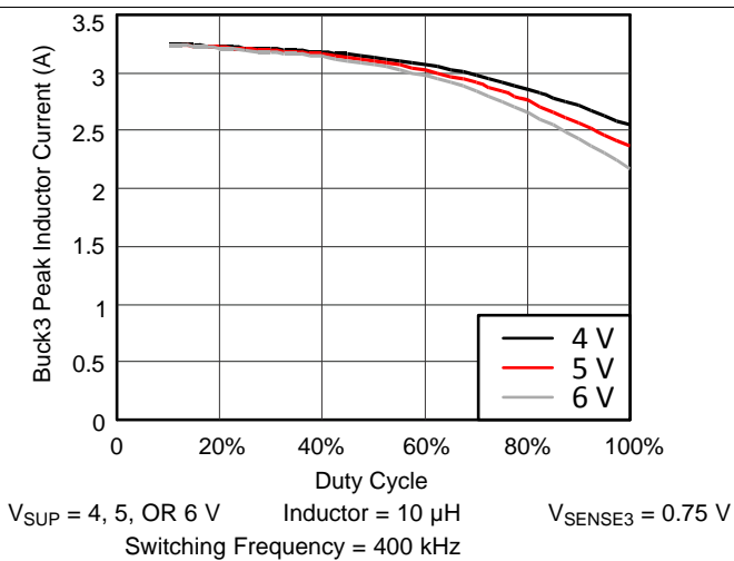
图 13. Buck3 Maximum Peak Inductor Current vs Duty Cycle
