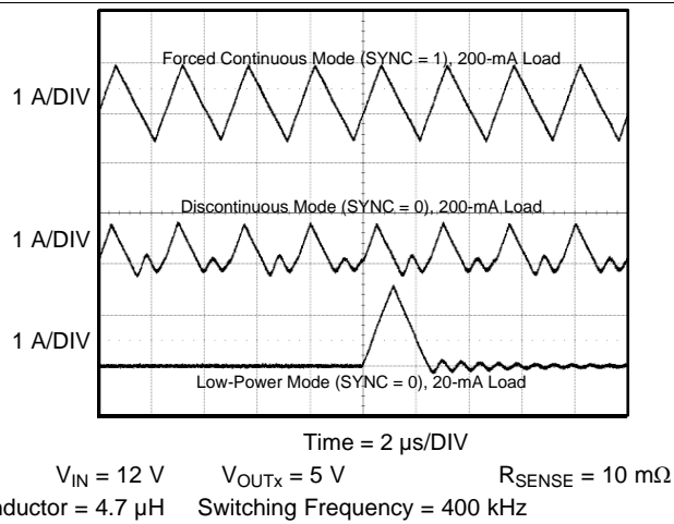
图 7. Inductor Currents (Buck1 and Buck2)
