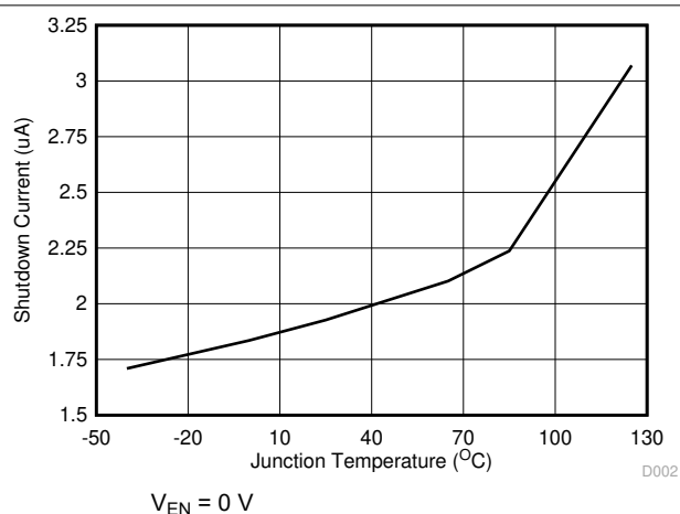
图 6-2. Shutdown Current vs Temperature
