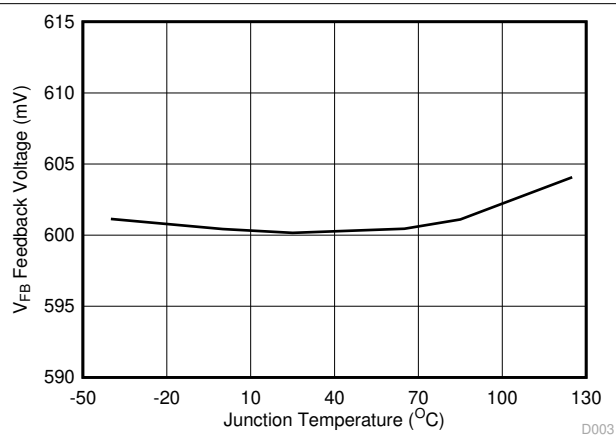
图 6-3. Feedback Voltage vs Junction Temperature
