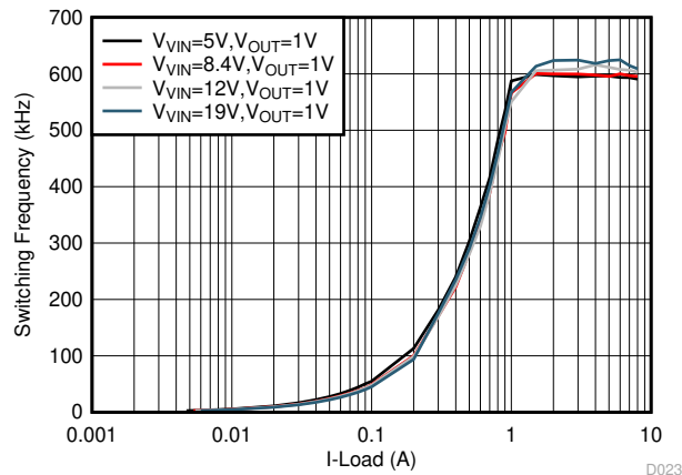
图 6-17. F_{SW} Load Regulation, Eco-mode, F_{SW} = 600 kHz
