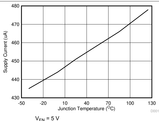
图 6-1. Supply Current vs Junction Temperature
