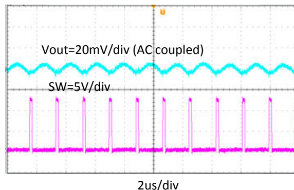
图 8-9. Output Voltage Ripple, I_{OUT} = 8\text{ A}
