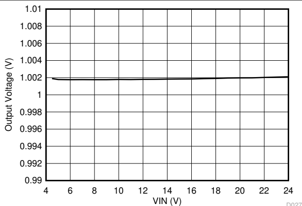
图 8-6. Line Regulation, I_{OUT} = 0.01\text{ A}
