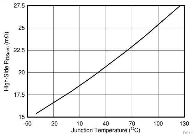
图 6-6. High-Side R_{\text{DS(on)}} vs Junction Temperature
