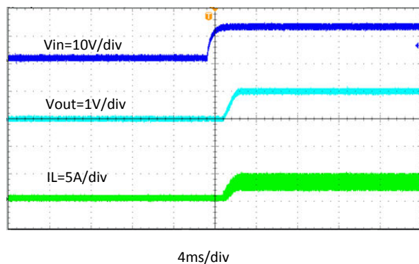
图 8-12. Start Up Relative to V_{IN} Rising, I_{OUT} = 4\text{ A}
