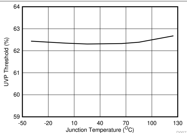
图 6-9. UVP Threshold vs Junction Temperature
