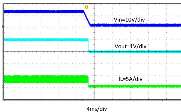
图 8-13. Start Up Relative to V_{IN} Falling, I_{OUT} = 4\text{ A}
