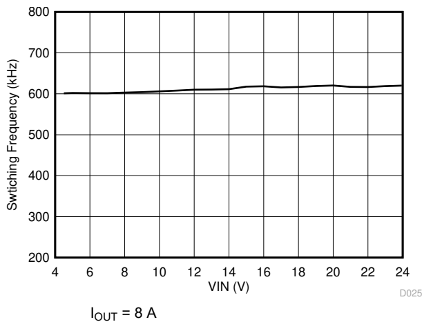
图 8-4. Switching Frequency vs Input Voltage
