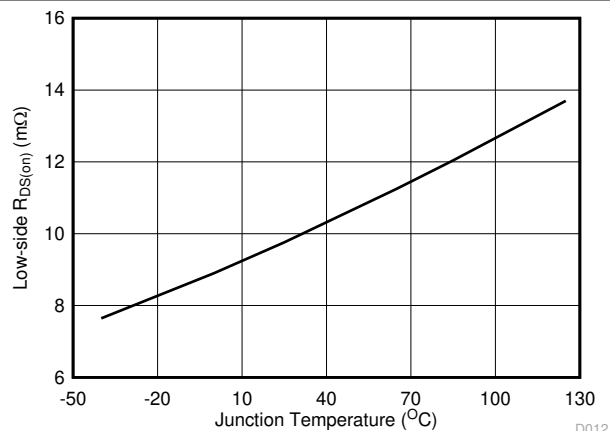
图 6-7. Low-Side R_{DS(on)} vs Junction Temperature
