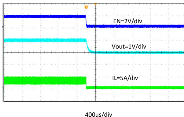
图 8-11. Shut-down Through EN, I_{OUT} = 4\text{ A}
