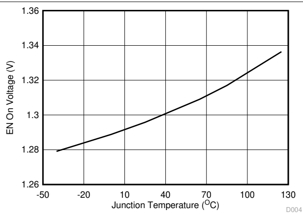
图 6-4. Enable On Voltage vs Junction Temperature
