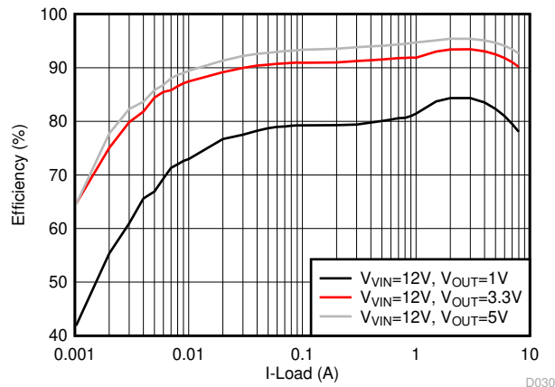
图 6-15. Efficiency, Eco-mode, F_{SW} = 1 MHz
