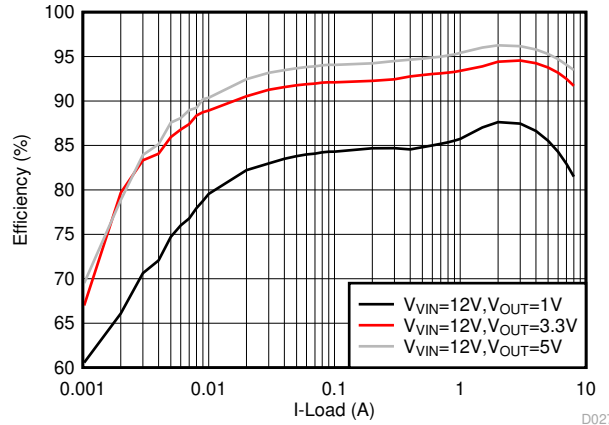
图 6-13. Efficiency, Eco-mode, F_{SW} = 600 kHz
