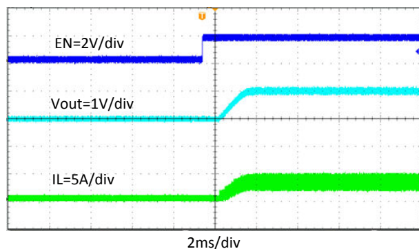
图 8-10. Start-Up Through EN, I_{OUT} = 4\text{ A}
