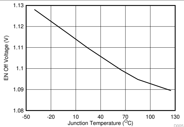
图 6-5. Enable Off Voltage vs Junction Temperature
