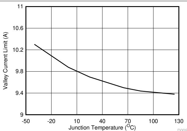
图 6-11. Valley Current Limit vs Junction Temperature
