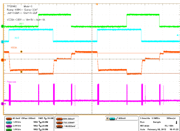
Figure 14. Mode=8, I_{OUT} = 0 A, VID Transitioning
