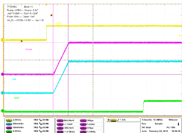
Figure 18. Mode= 8, I OUT = 3 A, Soft-Start
