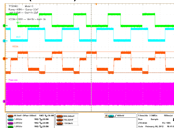
Figure 15. Mode=8, I_{OUT} = 3\text{ A} , VID Transitioning
