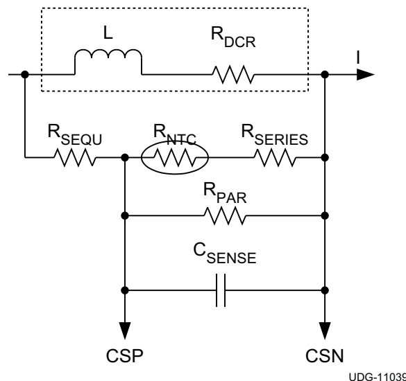
Figure 70. Typical DCR Sensing Circuit
