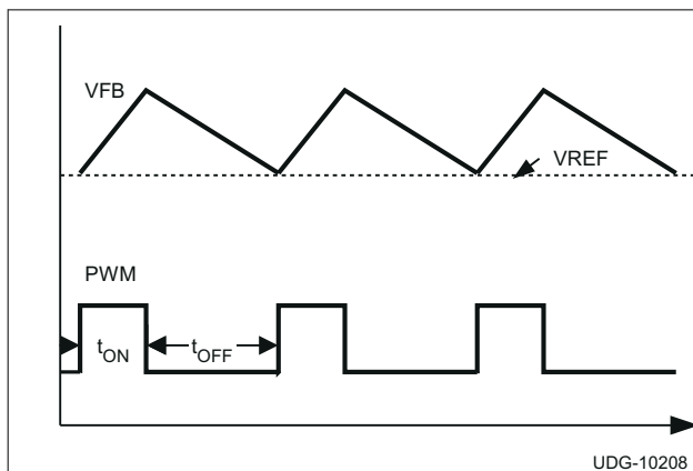
图 6-1. On-Time Control Without Ramp Compensation
