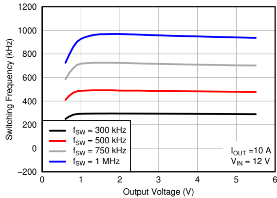
图 5-9. Switching Frequency vs Output Voltage
