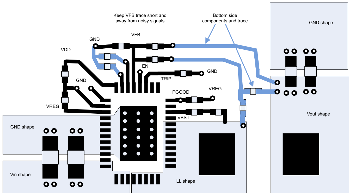
图 7-17. Layout Recommendation
