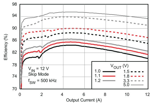
图 5-14. Efficiency vs Output Current
