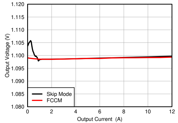
图 5-10. Output Voltage vs Output Current
