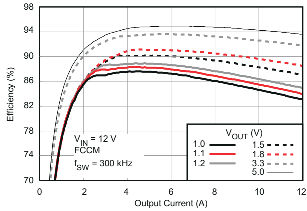
图 5-13. Efficiency vs Output Current
