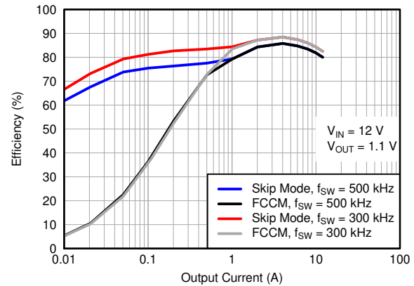
图 5-12. Efficiency vs Output Current, Inductor: IN06155
