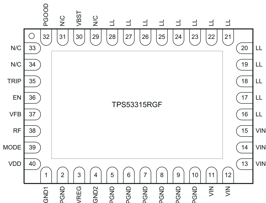
图 4-1. RGF Package 40-Pin VQFN With Exposed Thermal Pad Top View
