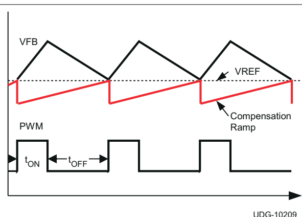
图 6-2. On-Time Control With Ramp Compensation
