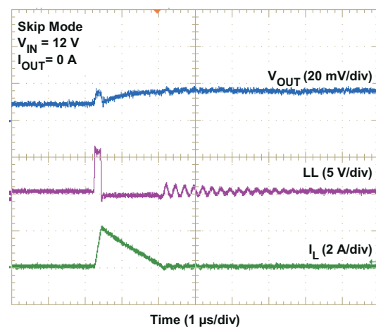
图 7-10. 1.1-V Output Skip Mode Steady-State Operation
