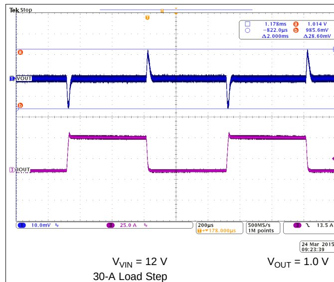
Figure 109. Transient Response
