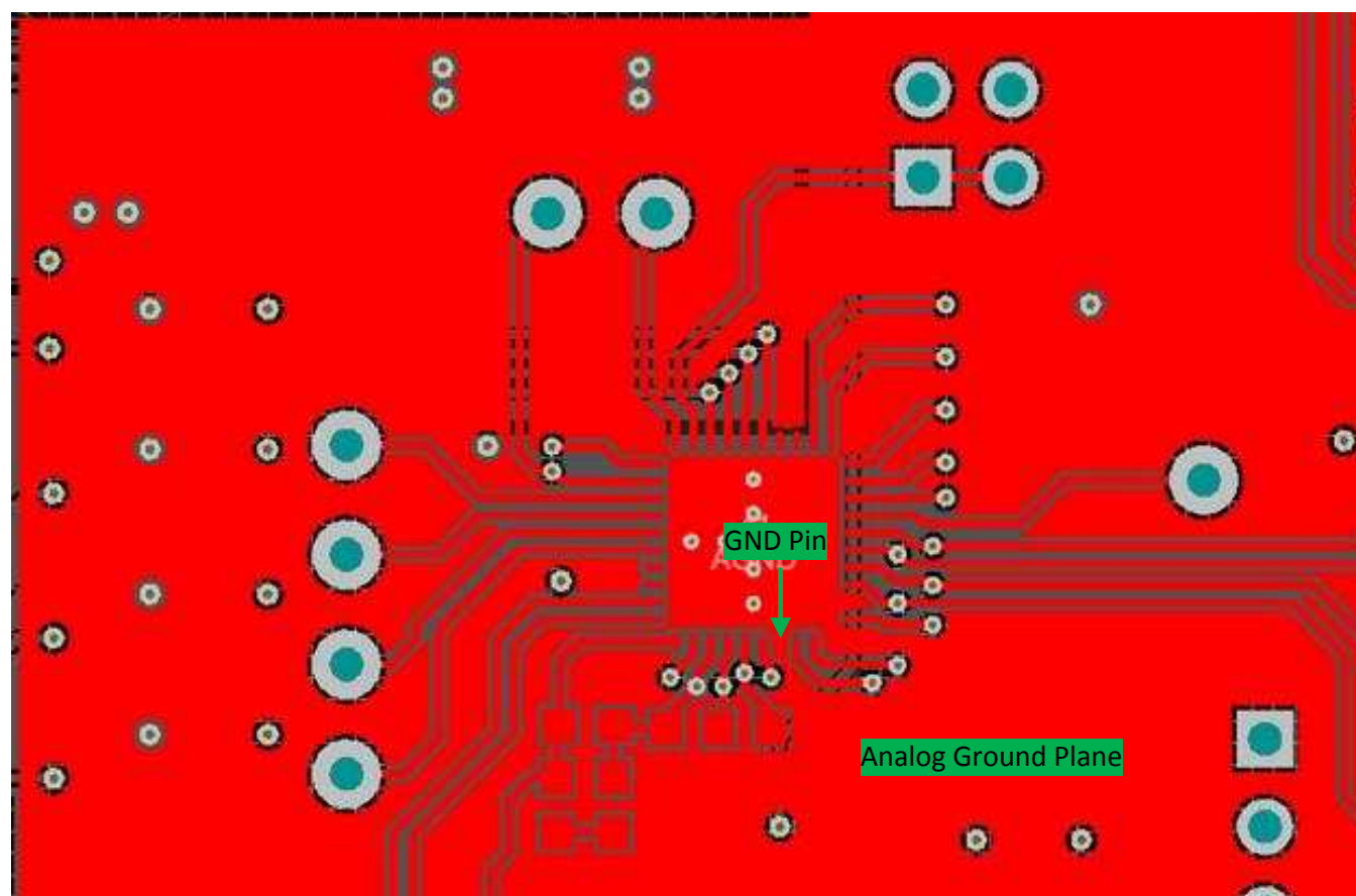
图 123. Layout Example for TPS53647 Grounding
