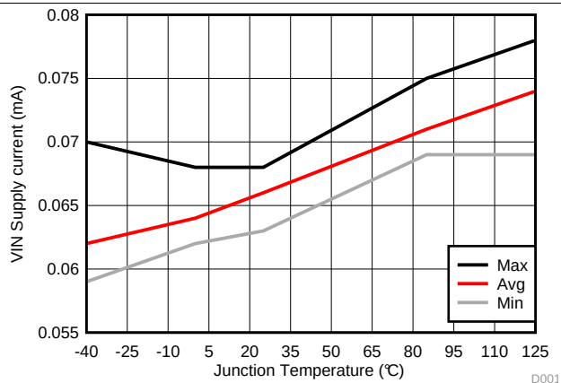
图 1. VIN Supply Current vs Junction Temperature
