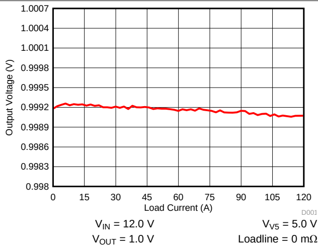
Figure 103. Load Regulation
