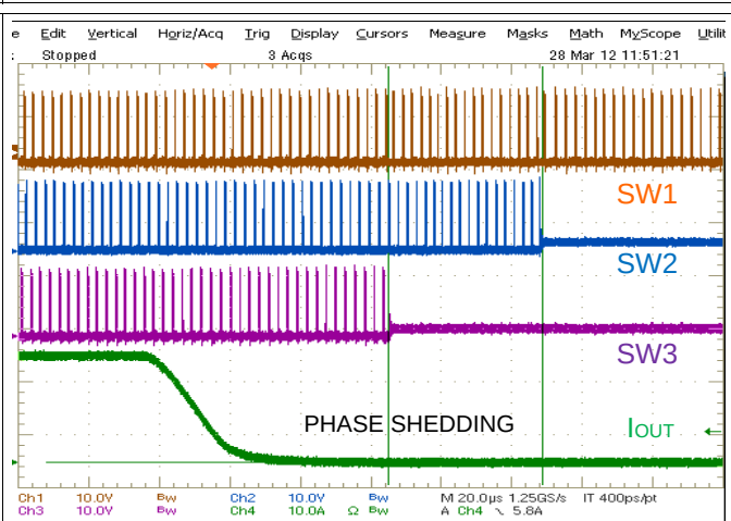
Figure 116. Phase Shedding
