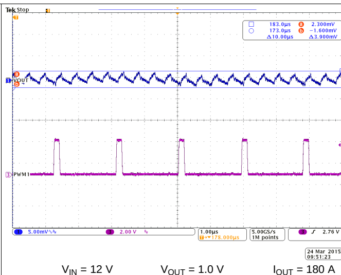
Figure 108. Output Ripple
