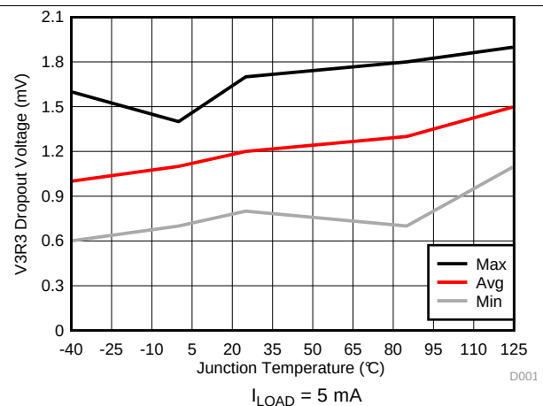
图 6. V3R3 Load Regulation vs Junction Temperature
