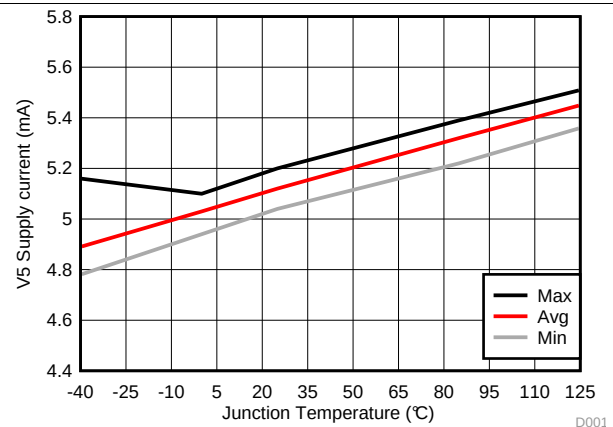
图 2. V5 Supply Current vs Junction Temperature
