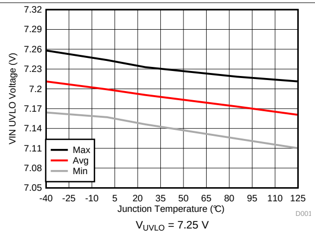
图 3. VIN UVLO Voltage vs Junction Temperature
