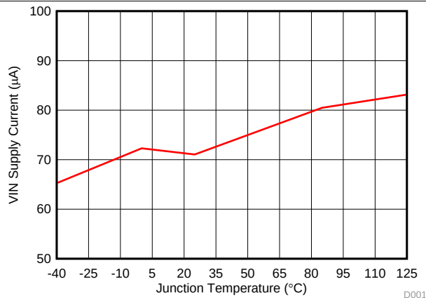
图 1. VIN Supply Current vs Junction Temperature
