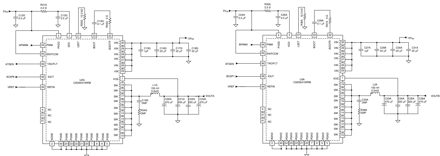
图 8-3. Powerstages Schematic (2/2)
