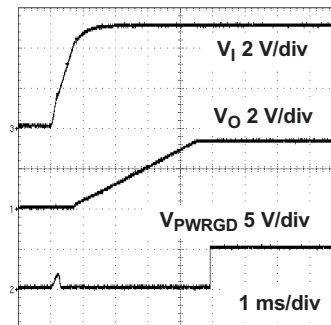
Figure 24. Slow-Start Timing
