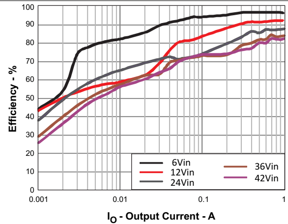
Figure 47. Light-Load Efficiency
