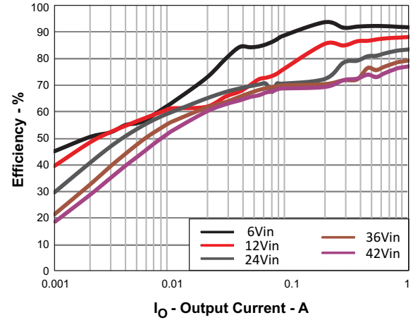
Figure 45. Light-Load Efficiency
