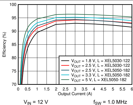
图 6-5. Efficiency vs Output Current - 1.8-V to 5.0-V Output
