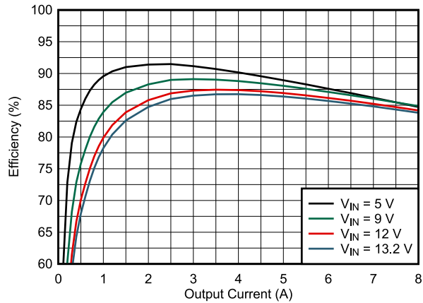
图 8-24. Efficiency
