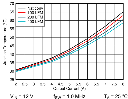
图 6-8. Junction Temperature vs Output Current – 3.3-V Output
