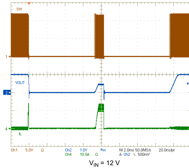
图 8-22. Overcurrent Protection – Hiccup and Recover
