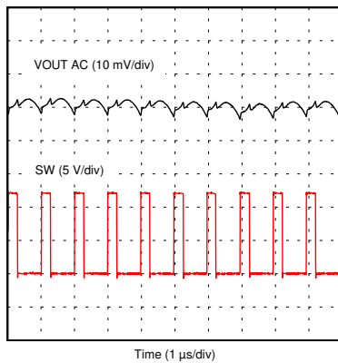
图 8-35. Output Ripple – No Load
