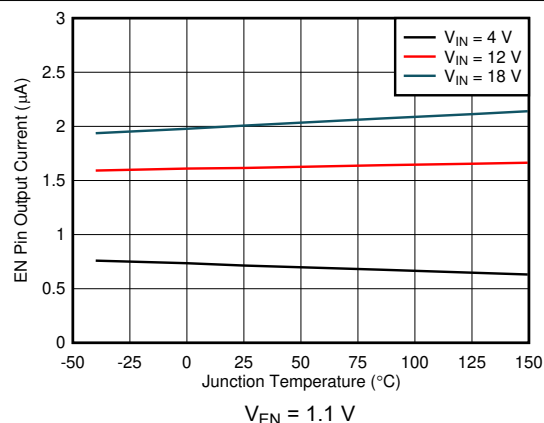
图 6-10. EN Pin Current vs Junction Temperature
