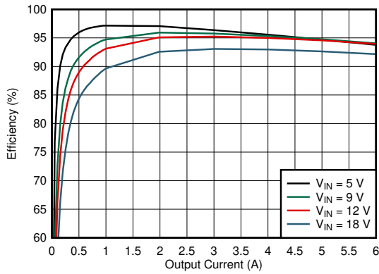
图 8-31. Efficiency
