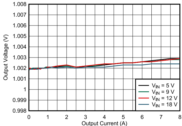
图 8-5. Load Regulation
