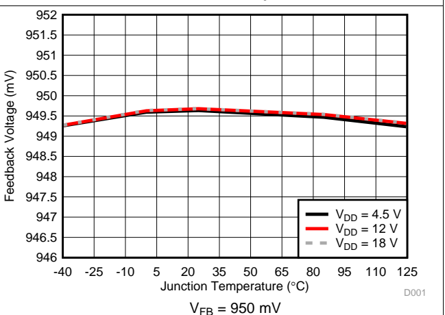
Figure 6. Feedback Voltage vs. Junction Temperature
