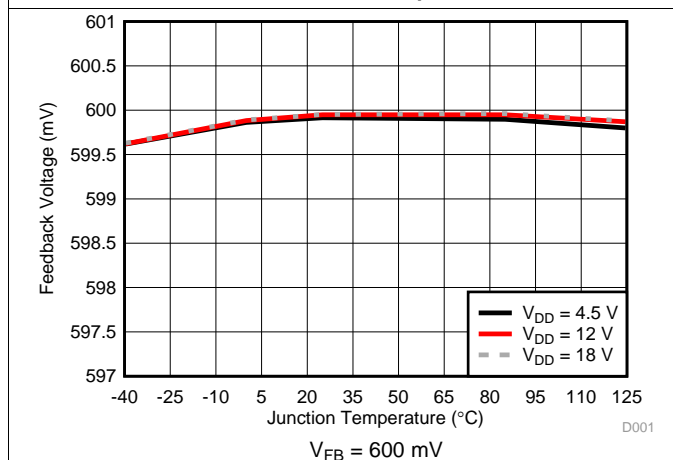
Figure 5. Feedback Voltage vs. Junction Temperature
