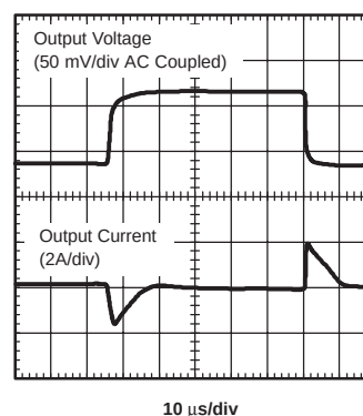
LOAD TRANSIENT RESPONSE
