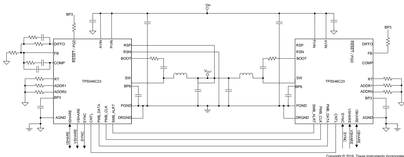
图 23. 2-Phase Application
