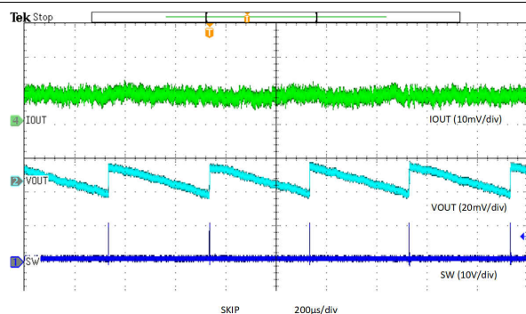
图 8-24. Output Voltage Ripple, Skip, 0.01-A Load
