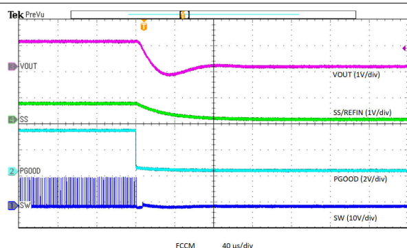
图 8-26. Overtemperature Protection in FCCM
