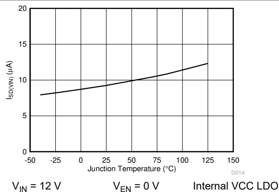
图 6-8. I_{SD}(V_{IN}) vs Junction Temperature
