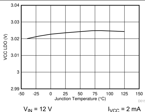
图 6-9. VCC LDO vs Junction Temperature
