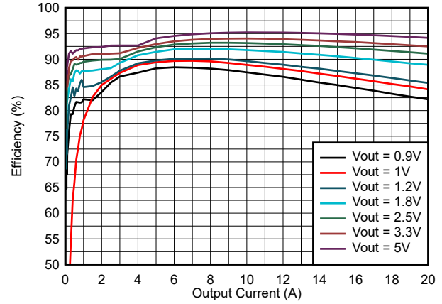
图 6-2. Efficiency vs Output Current, 12 V_{IN} , 800 KHz, DCM, V_{CC} = \text{EXT } 3.3 \text{ V}
