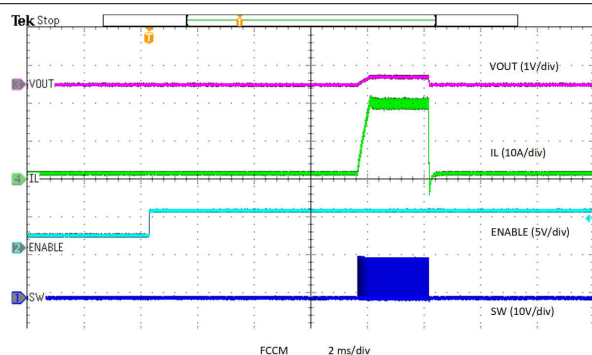
图 8-28. Enabled into Overcurrent
