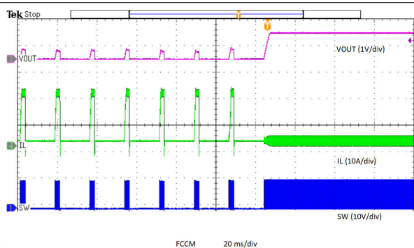
图 8-29. Hiccup Overcurrent
