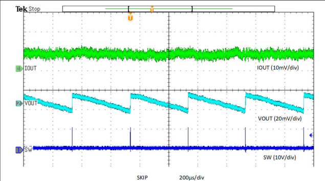
图 6-18. V OUT Ripple, Skip Mode, 10-mA Load
