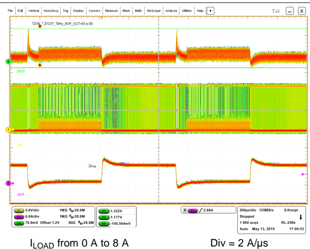
Figure 52. Auto-skip Mode Load Transient
