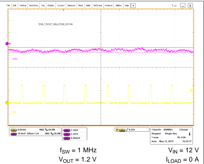
图 13. FCM Steady-State Operation
