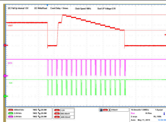
图 5-16. 6 Sequenced Events - I2C Write/Read with PEC
