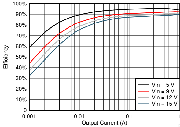
图 6-11. TPS561201 V_{OUT} = 3.3\text{ V} , Efficiency, L = 3.3\ \mu\text{H}
