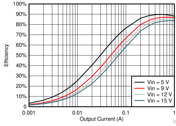
图 6-14. TPS561208 V_{OUT} = 1.5\text{ V} , Efficiency, L = 2.2\ \mu\text{H}
