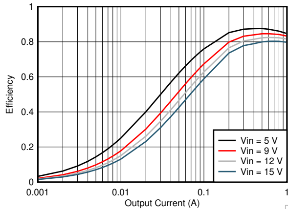
图 6-13. TPS561208 V_{OUT} = 1.05\text{ V} , Efficiency, L = 2.2\ \mu\text{H}
