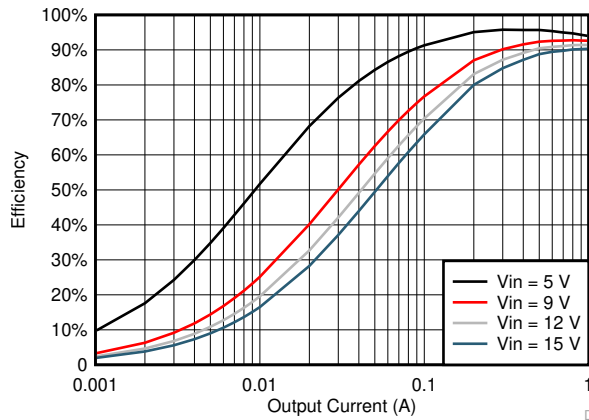
图 6-15. TPS561208 V_{OUT} = 3.3\text{ V} , Efficiency, L = 3.3\ \mu\text{H}
