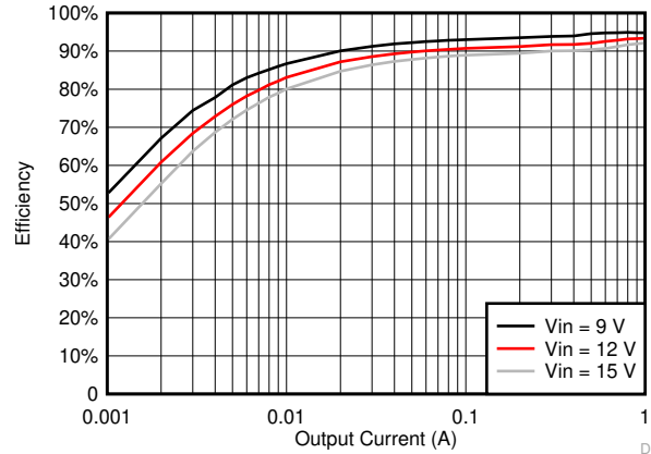
图 6-12. TPS561201 V_{OUT} = 5\text{ V} , Efficiency, L = 4.7\ \mu\text{H}
