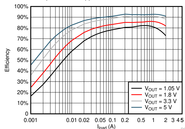
TPS562201 Efficiency
