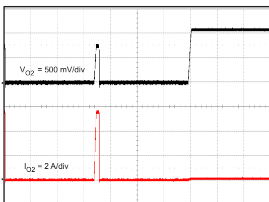
Figure 21. Hiccup Recover, Buck 2
