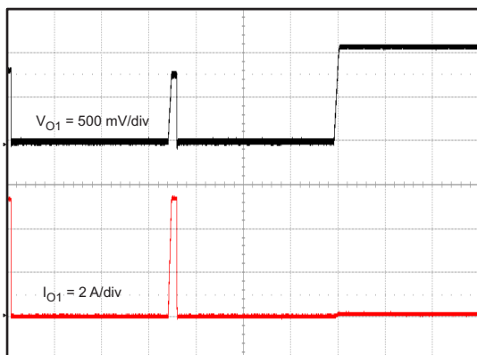
Figure 19. Hiccup Recover, Buck 1
