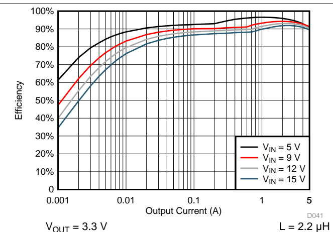
Figure 10. TPS565201 Efficiency vs Output Current
