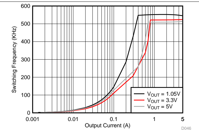
Figure 8. TPS565201 Switching Frequency vs Output Current
