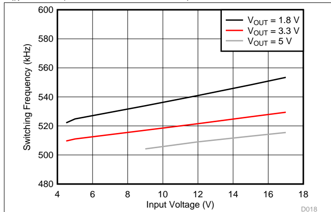
Figure 7. TPS565201 Switching Frequency vs Input Voltage
