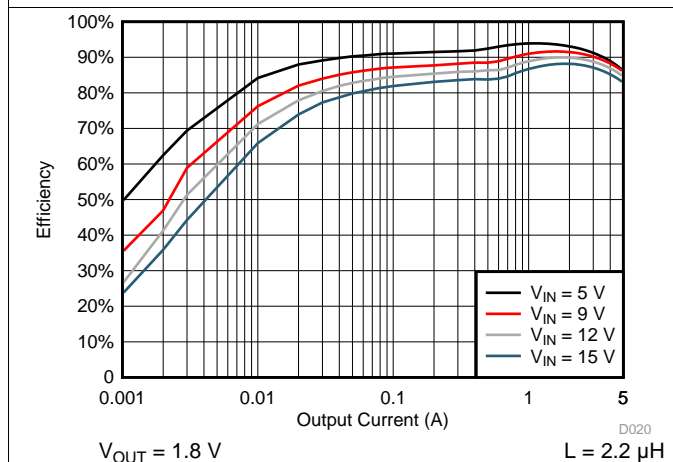
Figure 9. TPS565201 Efficiency vs Output Current
