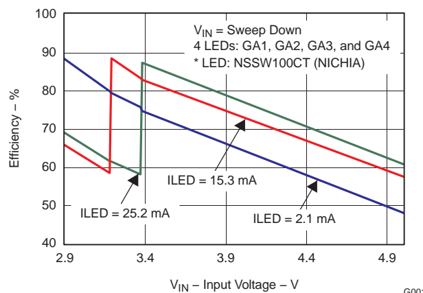
Figure 2. Characteristic Curve
