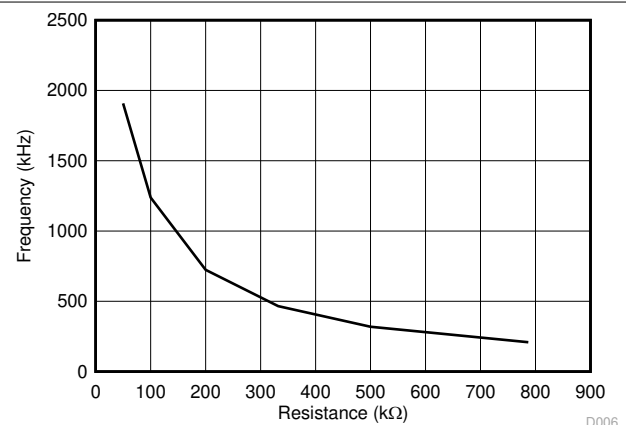
图 6-6. Switching Frequency vs Setting Resistance
