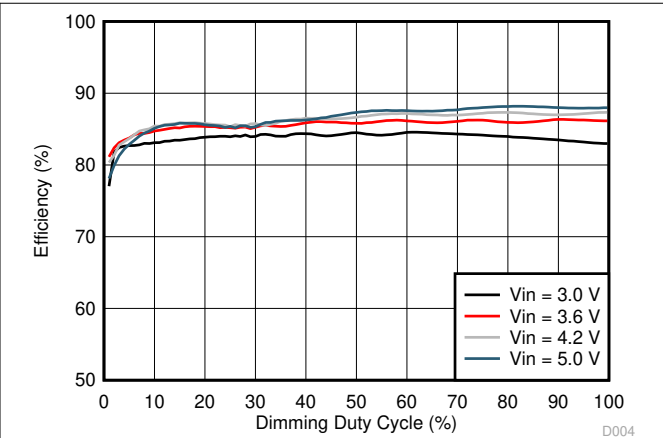
图 7-3. Efficiency vs Dimming Duty Cycle
