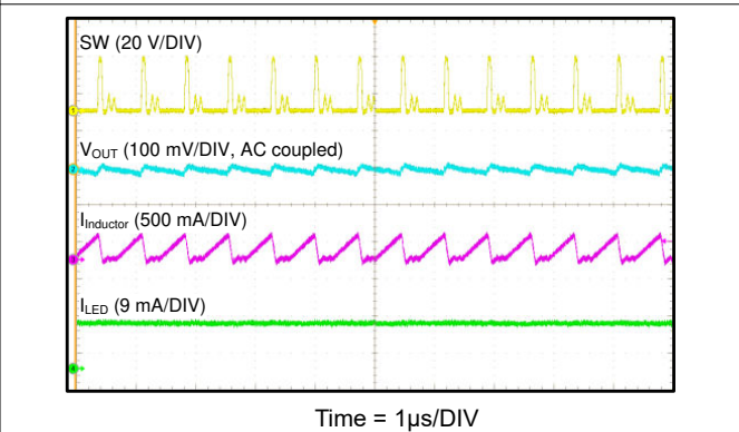
图 7-7. Switching-Dimming Duty = 50%
