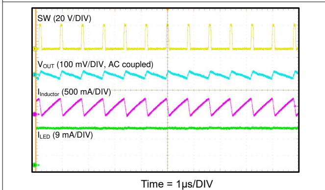
图 7-6. Switching-Dimming Duty = 100%
