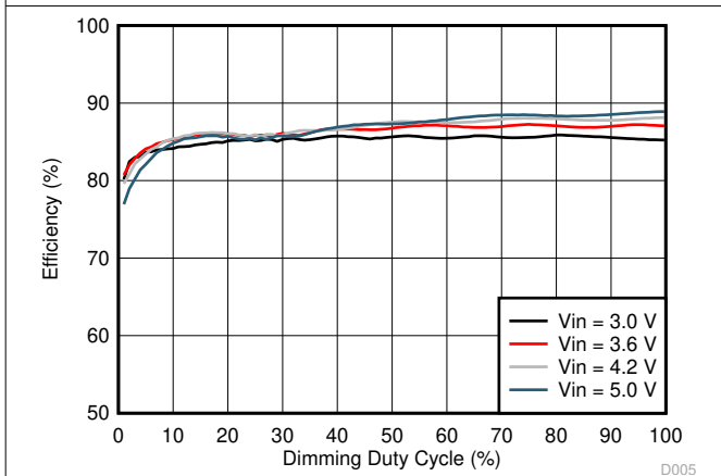
图 7-4. Efficiency vs Dimming Duty Cycle
