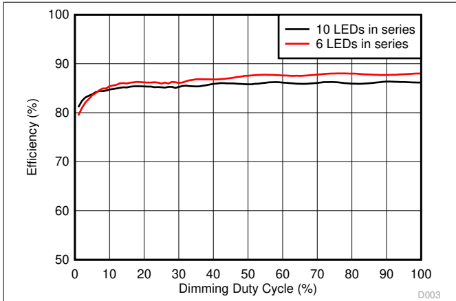
图 7-2. Efficiency vs Dimming Duty Cycle
