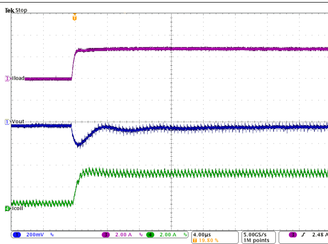
图 9-30. PWM-PSM-Transition
