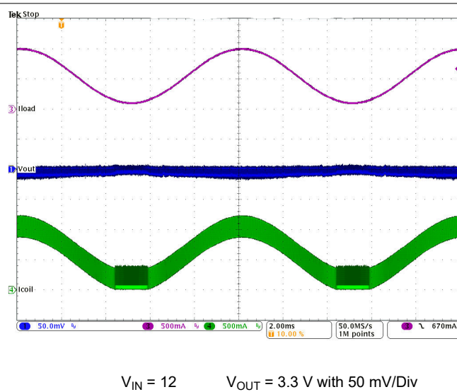
图 9-30. PWM-PSM-Transition
