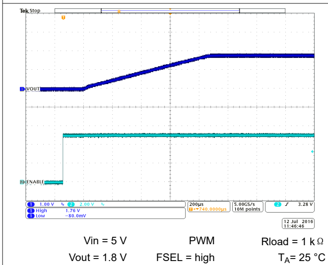
图 10-42. Start-Up Timing
