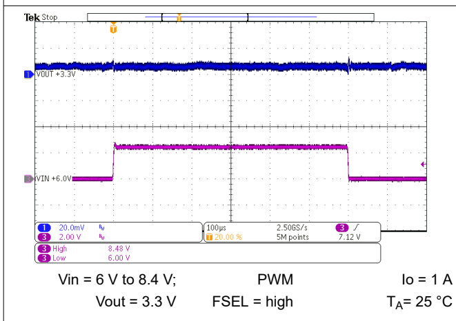
图 10-48. Line Transient Response
