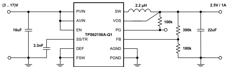
Figure 45. 2.5V/1A Power Supply
