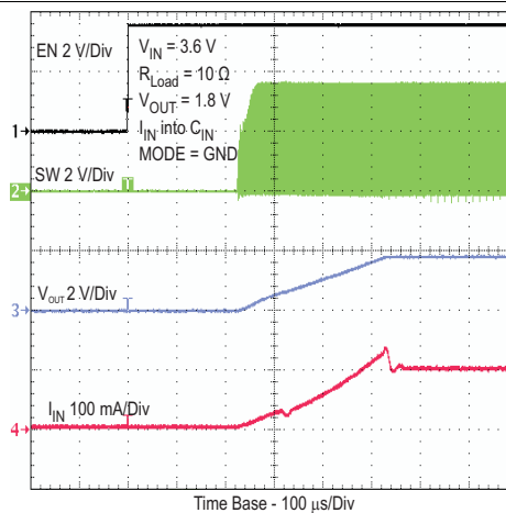
Figure 16. Start-UP Timing
