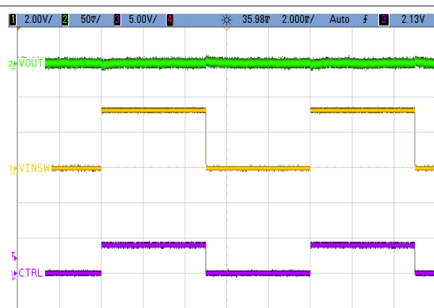
图 9-21. VINSW Operation and Control
