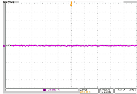
V_{OUT} = 0.6\text{ V} PWM T_A = 25^\circ\text{C} I_{OUT} = 4\text{ A} V_{IN} = 3.3\text{ V} BW = 20\text{ MHz}
