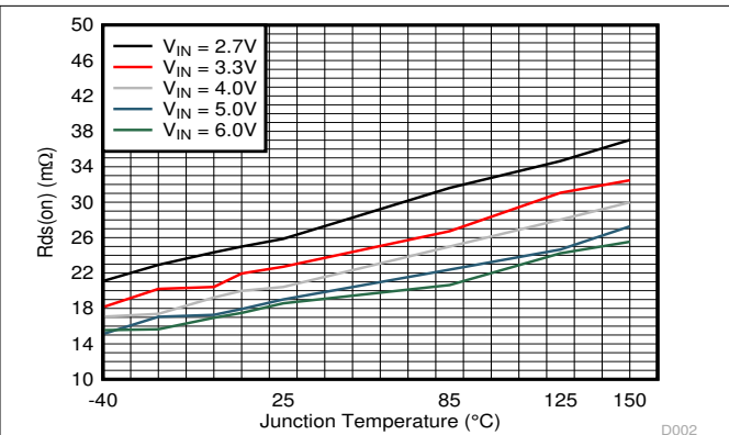
图 7-2. R_{ds(on)} of Low-side Switch
