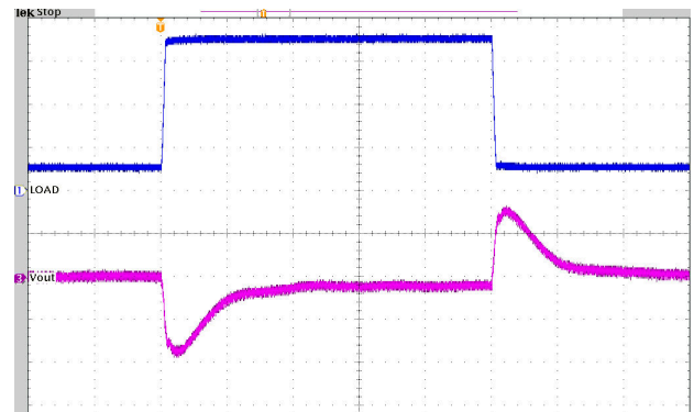
图 10-23. Load Transient Response
