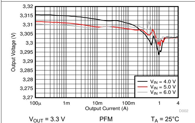
图 10-12. Output Voltage versus Output Current
