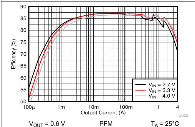
图 10-10. Efficiency versus Output Current
