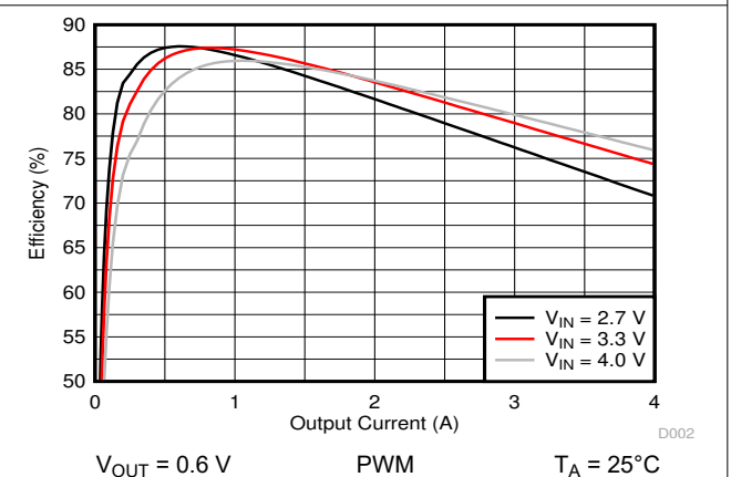
图 10-11. Efficiency versus Output Current
