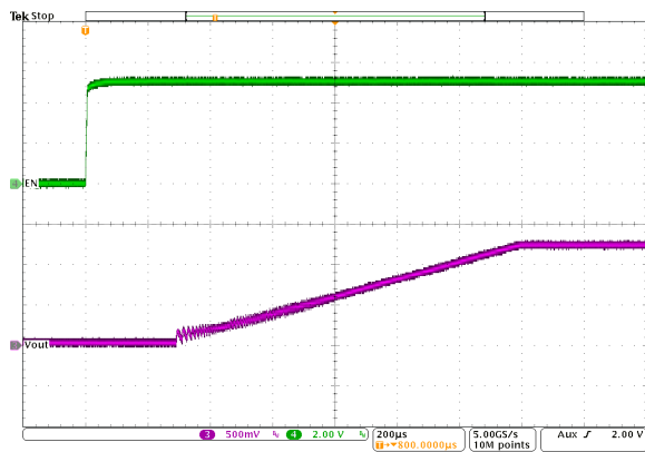
图 10-52. Start-Up Timing
