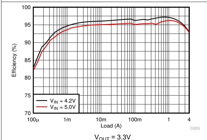
图 8-19. Efficiency
