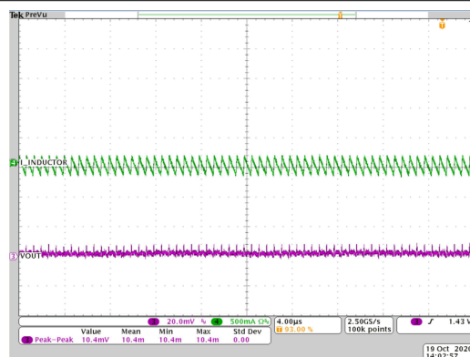
V_{IN} = 12V 2.5MHz FPWM I_O = 0.1A V_{OUT} = 1.2V L = 2.2 \mu H T_A = 25^\circ C
