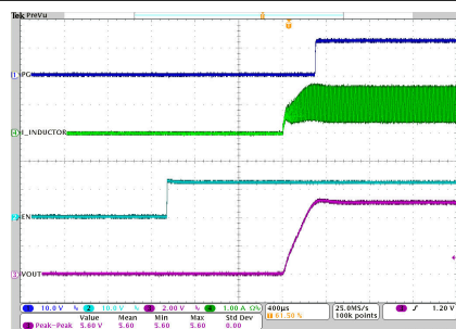
V_{IN} = 12V 1MHz 自动 PFM/PWM I_O = 1A V_{OUT} = 5V T_A = 25^\circ C
