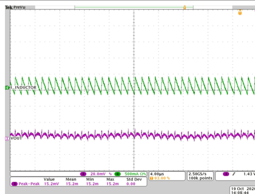
V_{IN} = 12V 1MHz FPWM I_O = 0.1A V_{OUT} = 1.2V L = 2.2 \mu H T_A = 25^\circ C
