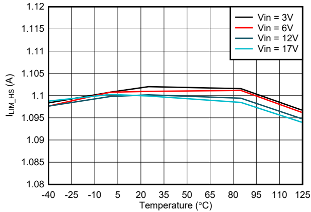
图 7-13. High-Side I_{LIM} vs Temperature
