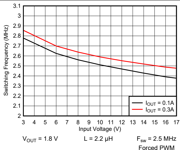
图 9-29. Switching Frequency vs Input Voltage
