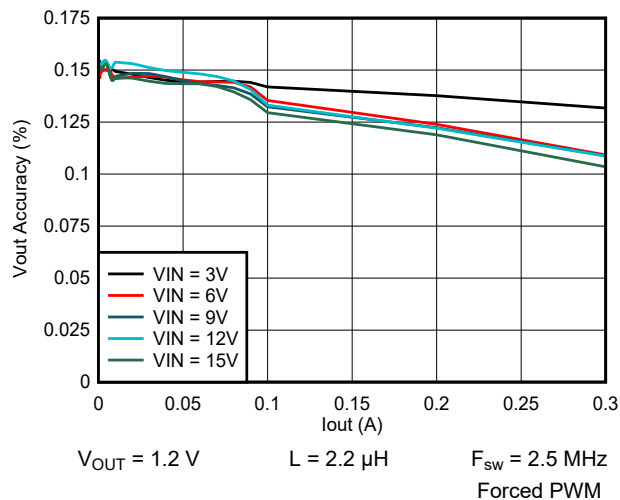
图 9-43. Output Voltage vs Output Current
