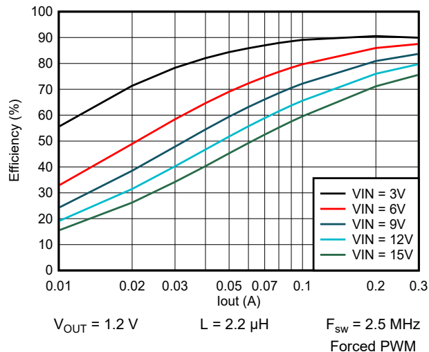
图 9-39. Efficiency vs Output Current
