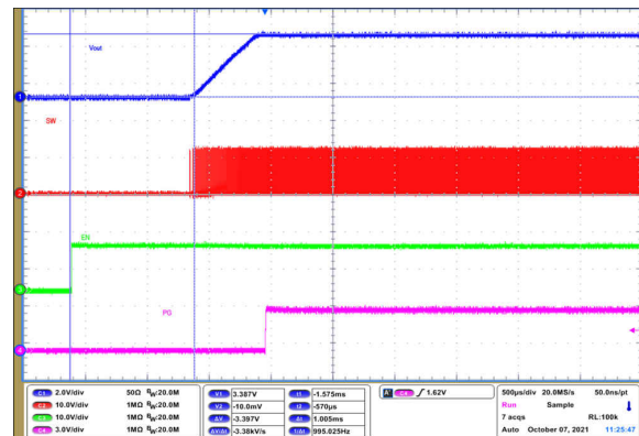
图 9-63. Start-Up Timing
