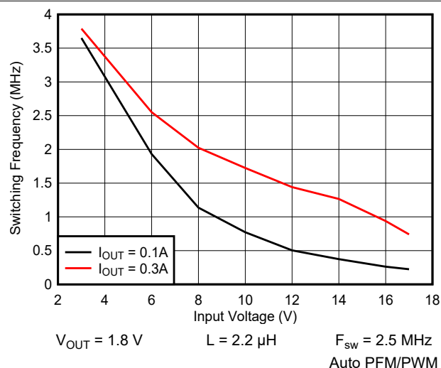
图 9-28. Switching Frequency vs Input Voltage
