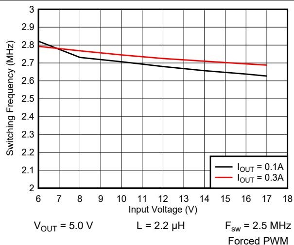
图 9-5. Switching Frequency vs Input Voltage
