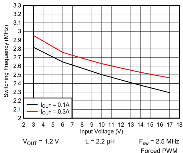
图 9-41. Switching Frequency vs Input Voltage
