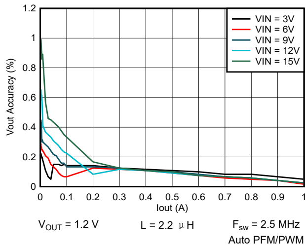
图 9-42. Output Voltage vs Output Current
