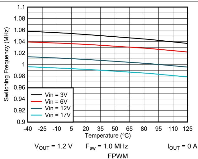
图 7-10. Switching Frequency vs Temperature
