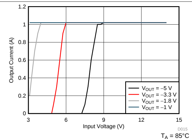
图 38. Maximum Output Current vs Input Voltage
