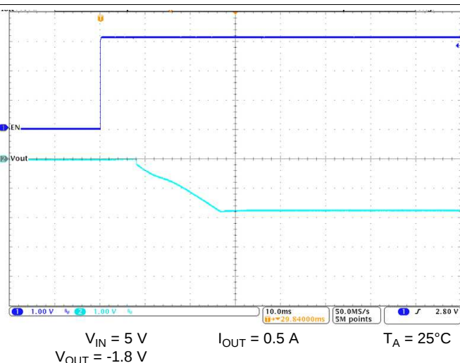
图 28. Start-Up Timing
