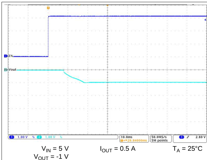
图 27. Start-Up Timing
