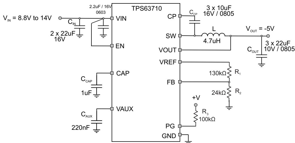
图 42. Typical Application for an Output Voltage of -5 V
