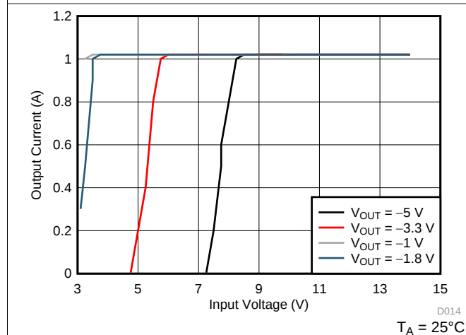
图 37. Maximum Output Current vs Input Voltage
