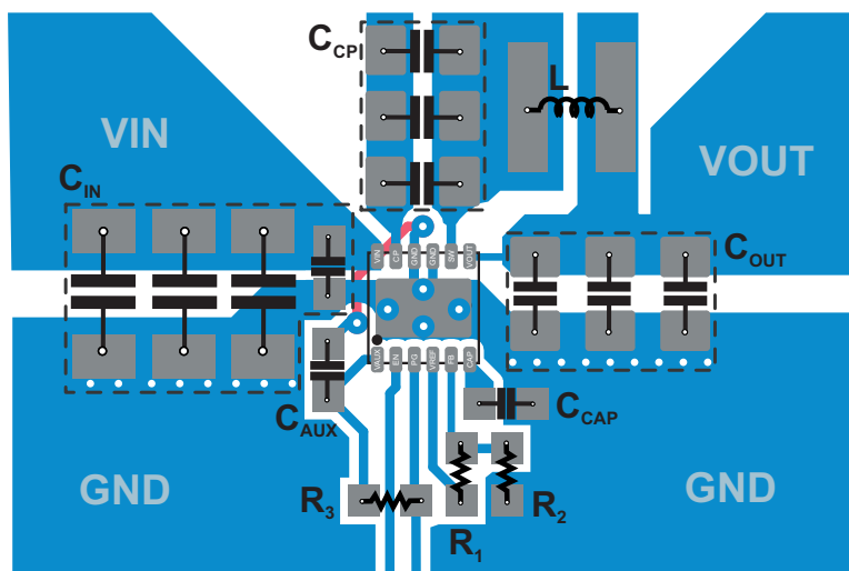
图 45. Recommended Layout
