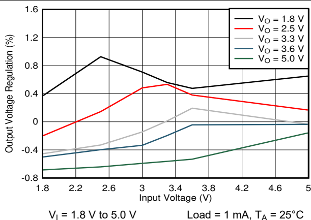
图 8-19. Line Regulation
