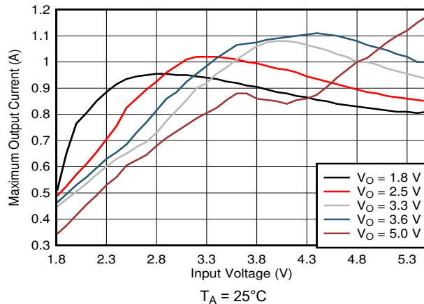
图 8-2. Typical Output Current Capability versus Input Voltage
