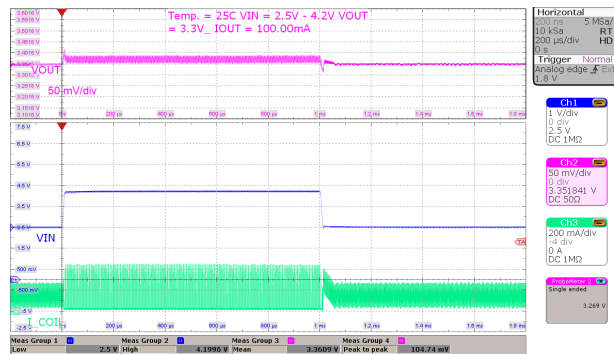
图 8-21. Line Transient, High Load
