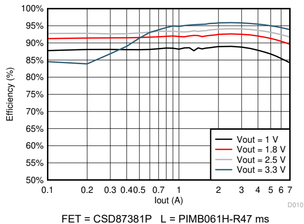
图 8-8. BUCK1 Efficiency at V_{IN} = 5\text{ V}
