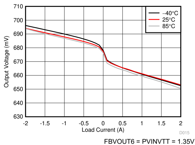
图 6-8. VTT LDO Regulation
