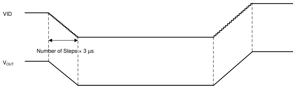
图 7-19. DVS Timing Diagram I (BUCKx_DECAY = 0)
