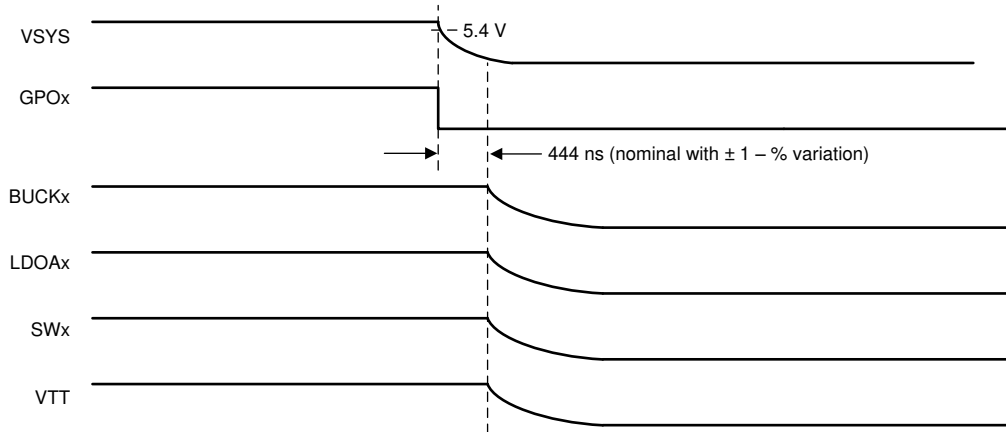
图 6-8. Emergency Shutdown Sequence
