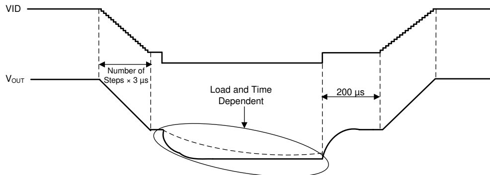
图 6-5. DVS Timing Diagram II (BUCKx_DECAY = 0b)
