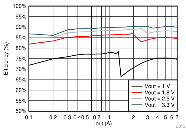
图 5-4. BUCK6 Efficiency at V_{IN} = 18V
