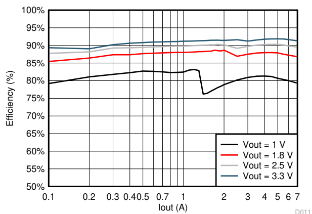
图 5-3. BUCK6 Efficiency at V_{IN} = 13V
