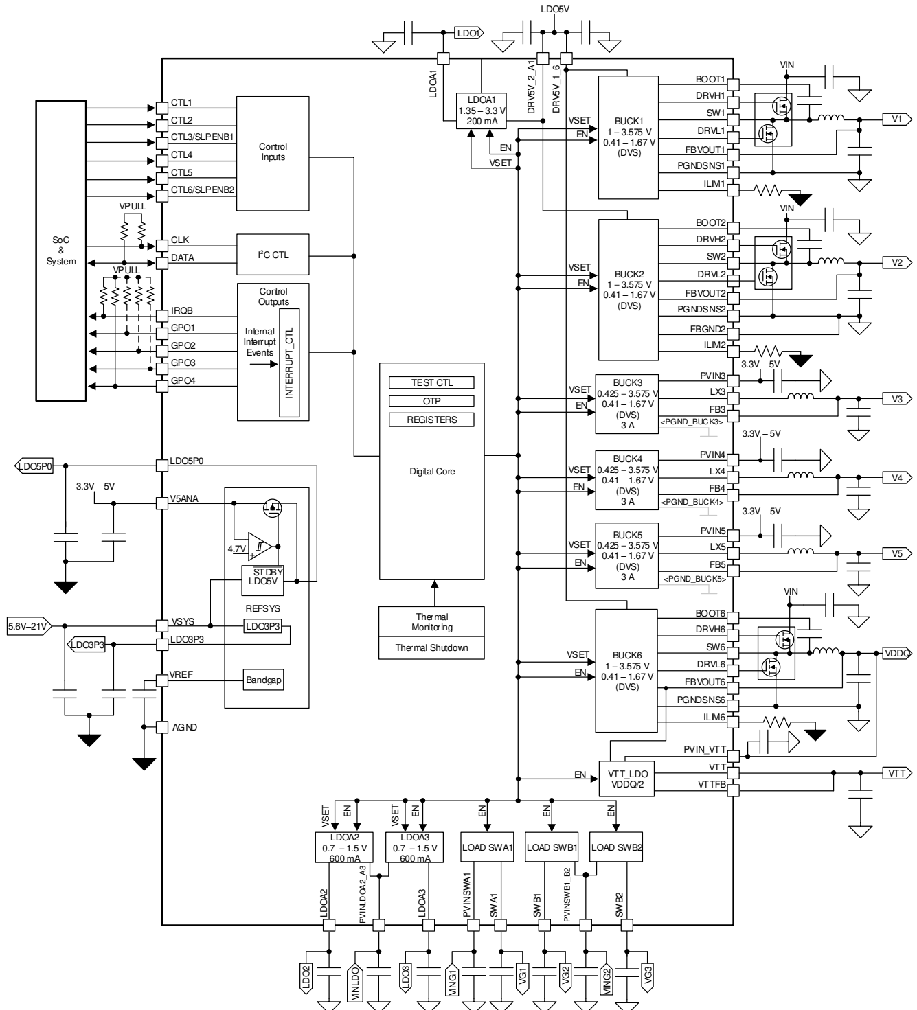
图 6-1. PMIC Functional Block Diagram
