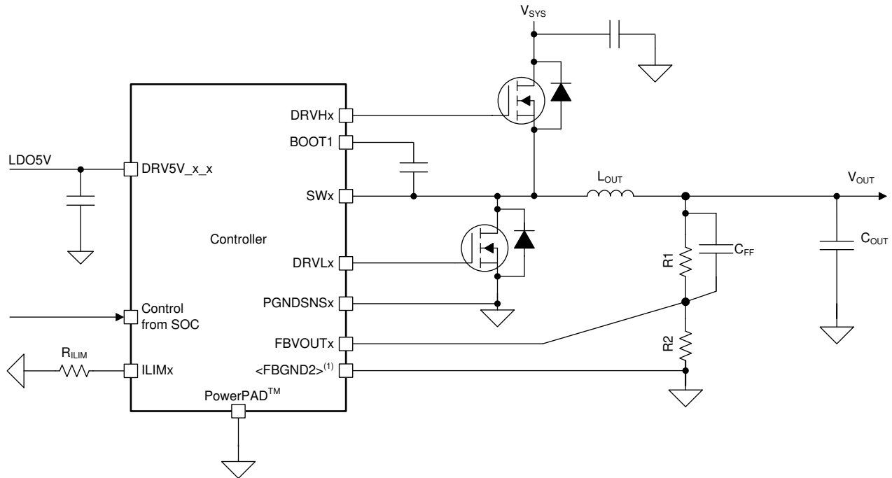
图 7-4. Controller Diagram With External Feedback Resistor
