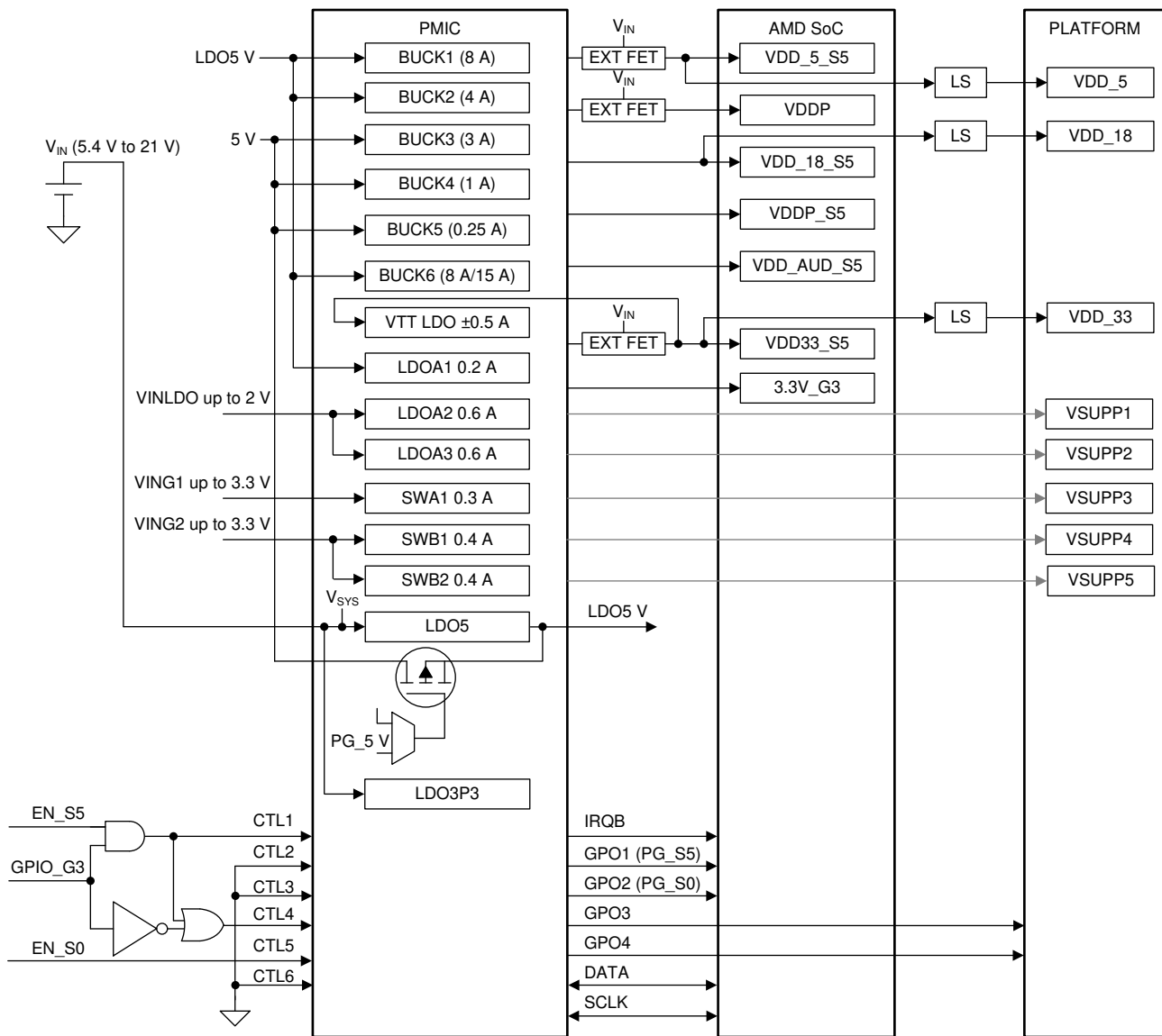
图 7-2. Typical Application Example
