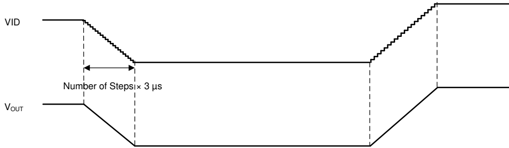
图 6-4. DVS Timing Diagram I (BUCKx_DECAY = 0b)
