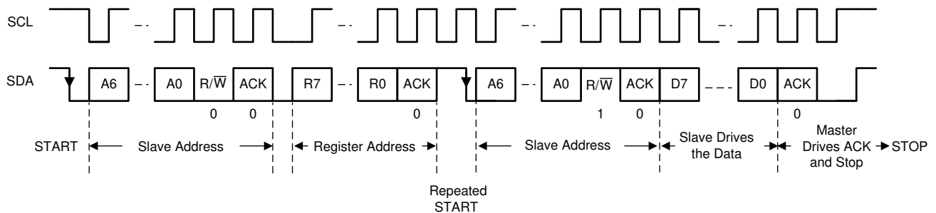
图 6-14. I²C Interface READ From TPS6508700 in F/S Mode (Only Repeated START is Supported)
