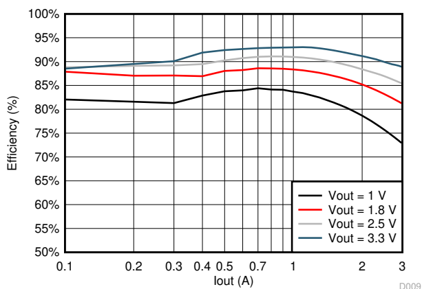
图 5-5. Converter Efficiency at V_{IN} = 5V
