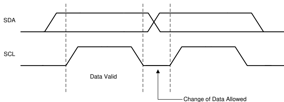
图 6-10. Bit Transfer on the I 2 C Bus
