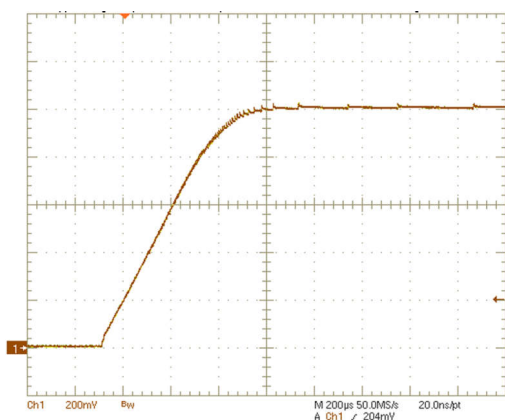
图 5-1. BUCK2 Controller Start Up to 1V by I 2 C
