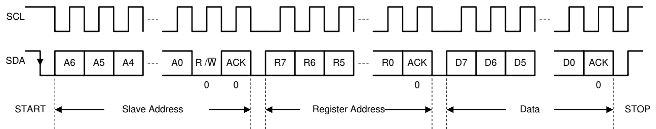
图 6-13. I²C Interface WRITE to TPS6508700 in F/S Mode
