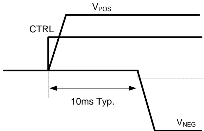
Figure 8. Start-up Sequence
