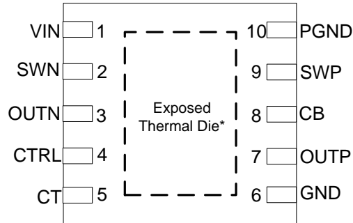
10 PIN TQFN PACKAGE (TOP VIEW)
