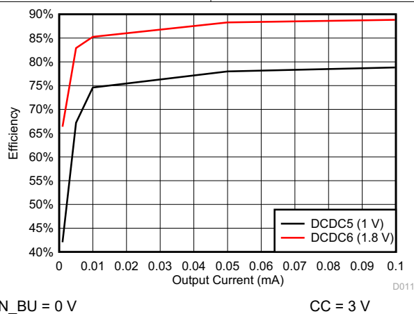
图 8-8. DCDC5/DCDC6 Efficiency
