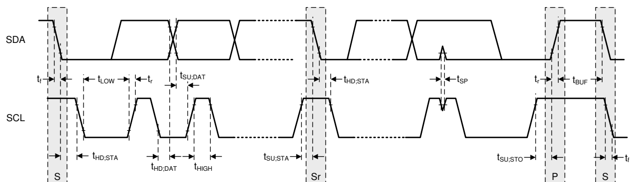
图 7-34. I²C Protocol and Transmission Timing I²C Data Transmission Timing
