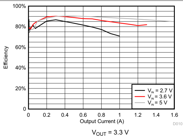
图 8-7. DCDC4 Efficiency
