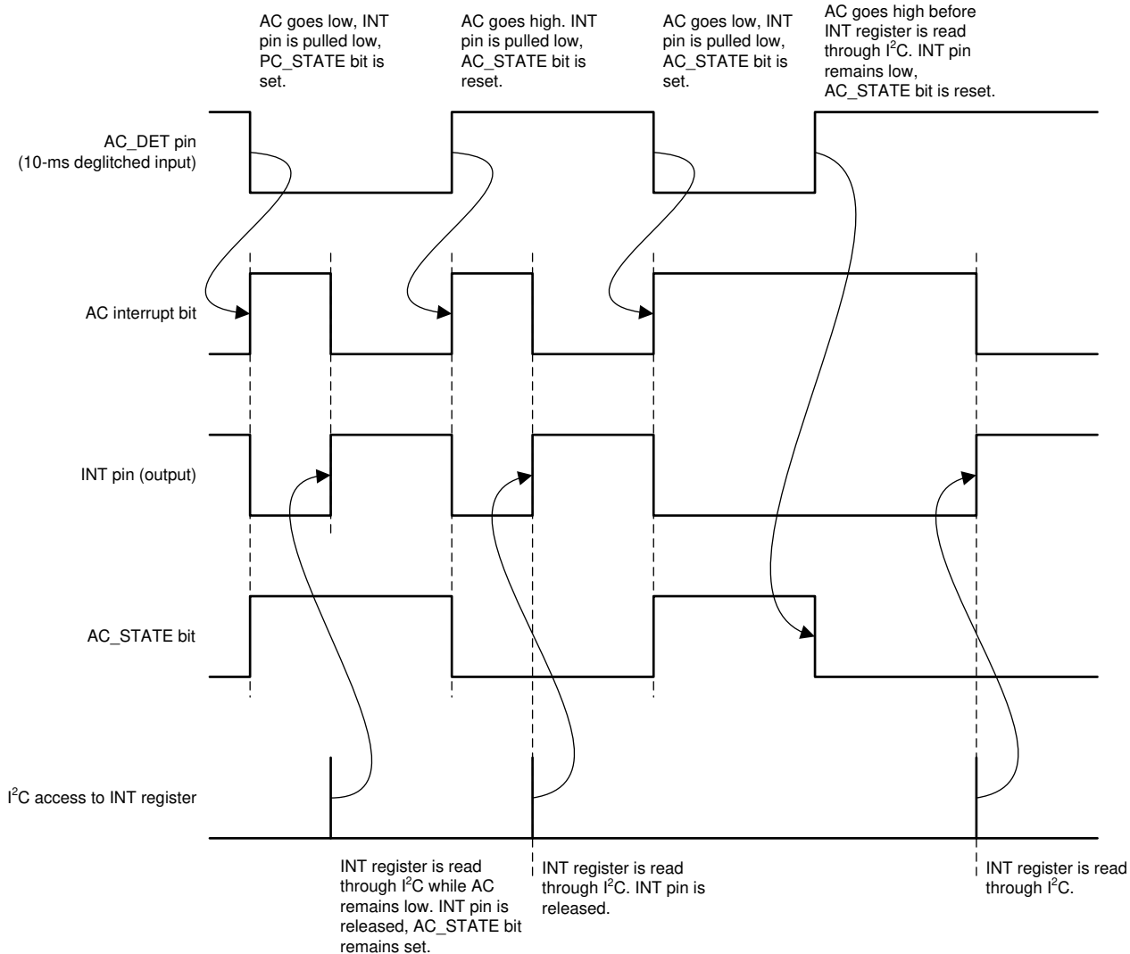
图 7-30. AC_STATE Pin
