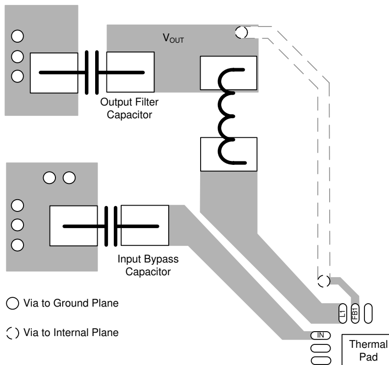
图 10-1. Layout Recommendation
