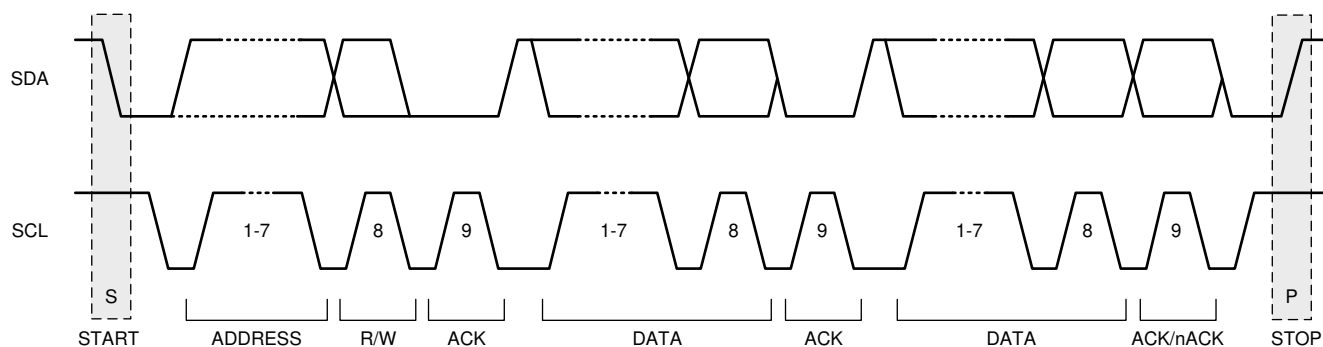
图 7-33. I²C Protocol and Transmission Timing I²C Start Stop and Acknowledge Protocol
