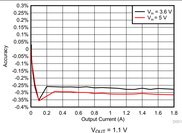
图 6-1. DCDC1 Accuracy
