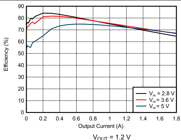
图 8-5. DCDC3 Efficiency
