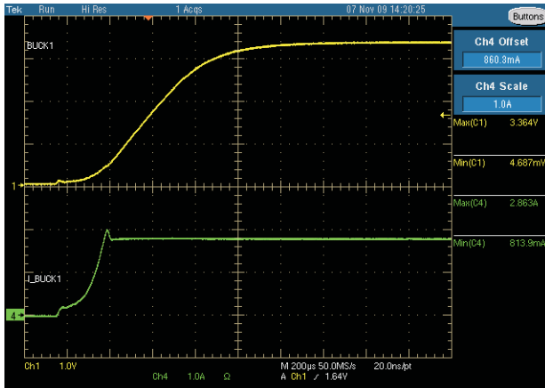
Figure 5. Start-Up V_{OUT} = 3.3\text{ V} , 2\text{ A}
